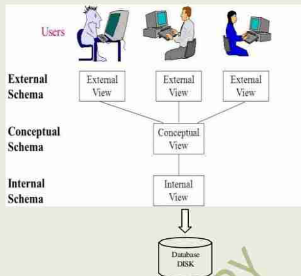
Figure 1.2 : Levels of Abstraction in a DBMS
