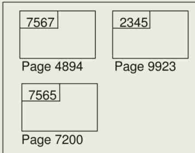
Database Buffer
