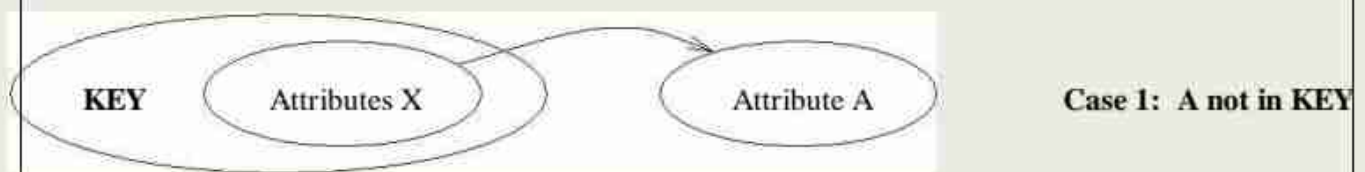
Figure 15.9 Partial Dependencies
