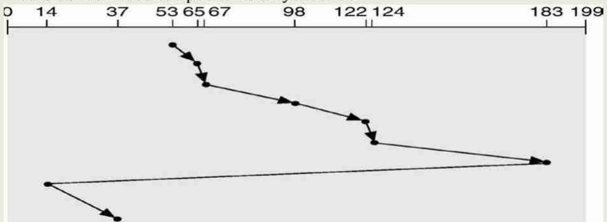
(C-LOOK disk scheduling)
