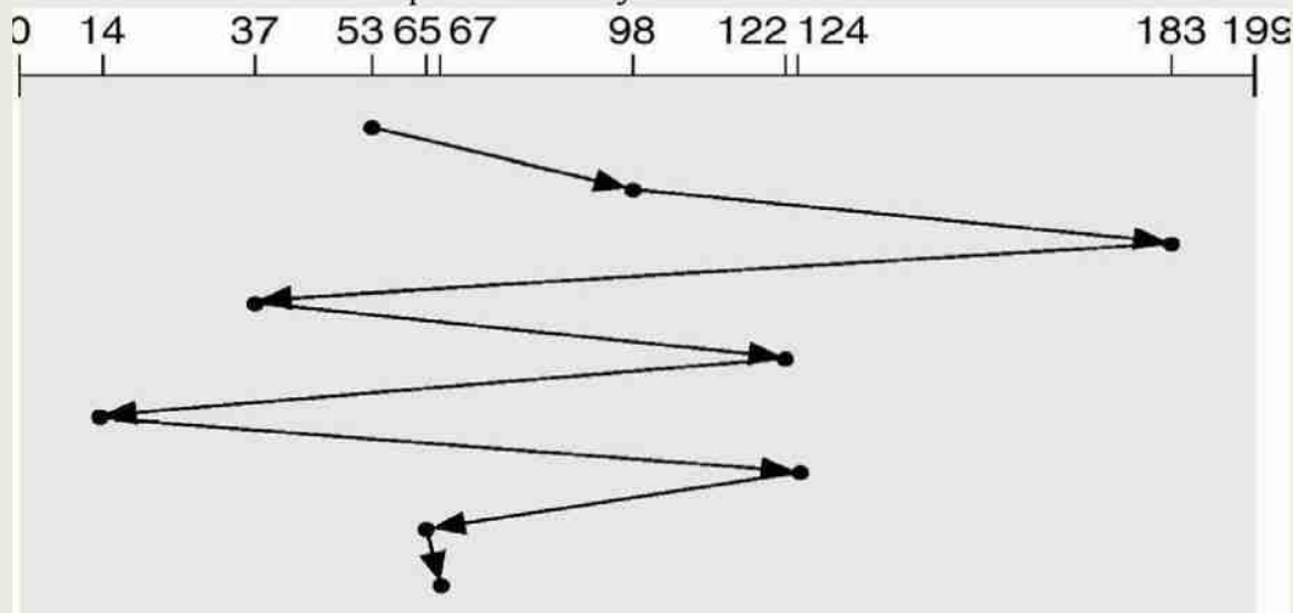
(FCFS disk scheduling)
