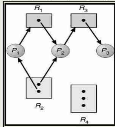
Example of a Resource Allocation Graph
