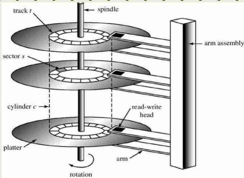
(Structure of Magnetic disks (Harddisk drive))
