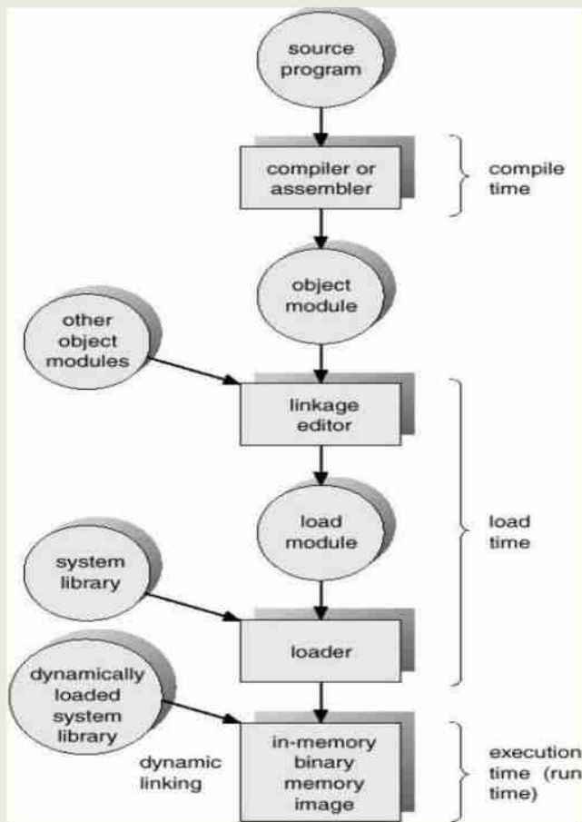
(Multistep processing of a user program.)
