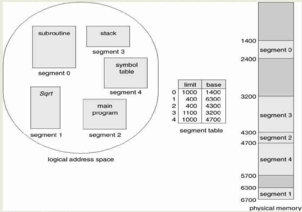
(Example of segmentation)
