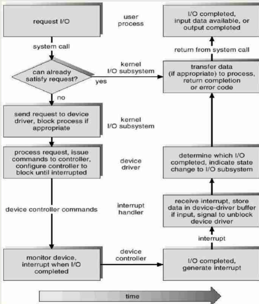
(The life cycle of an I/O request)
